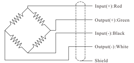
Wiring Diagram
