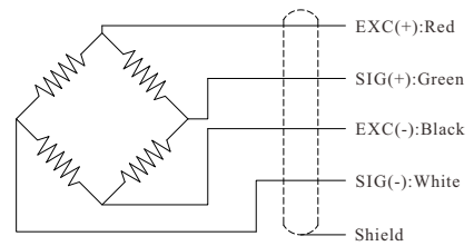
Wiring Diagram
