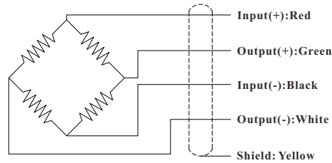
Wiring Diagram@Compression
